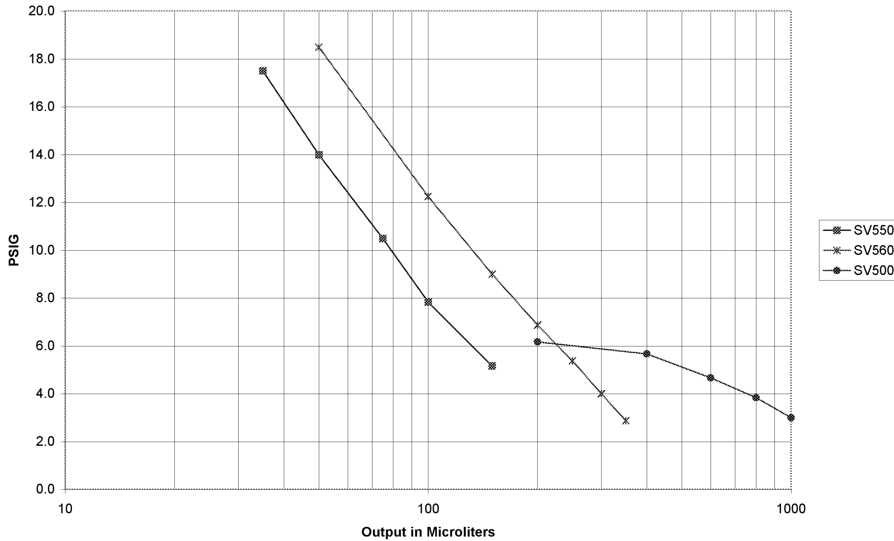
Output volume vs. Pressure
