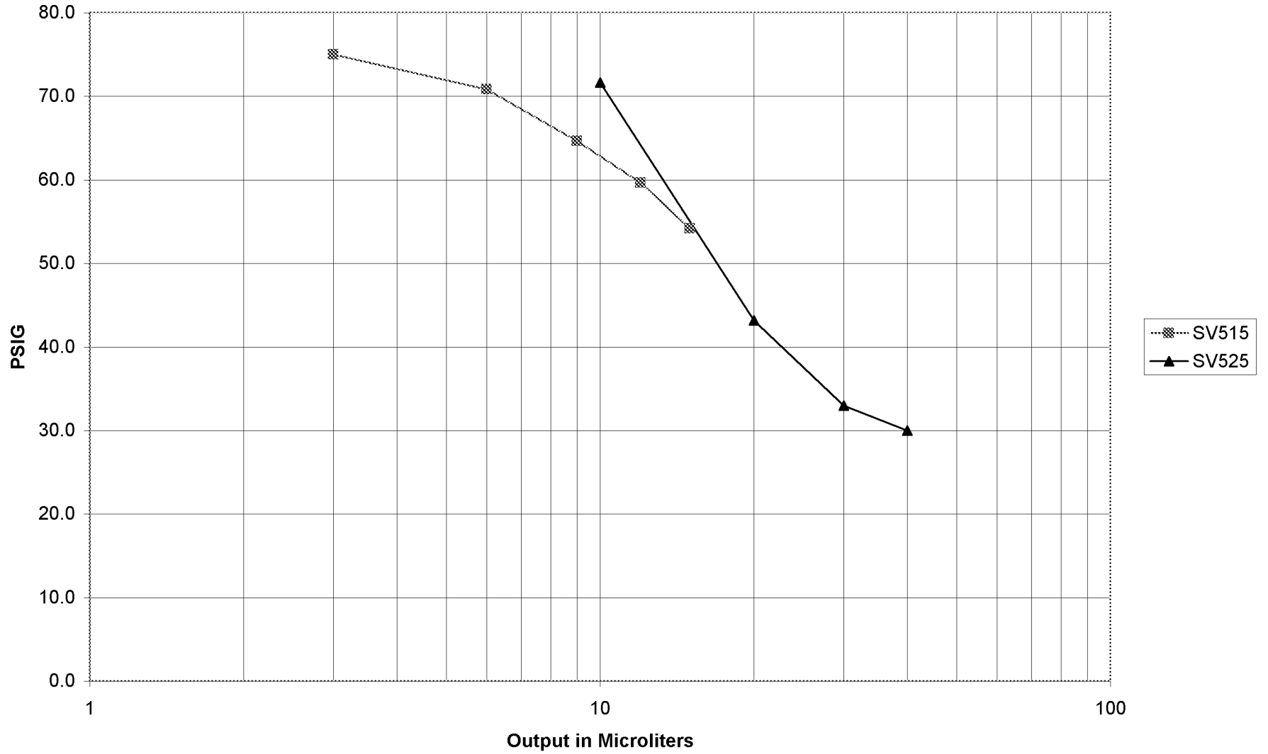
Output volume vs. Pressure
